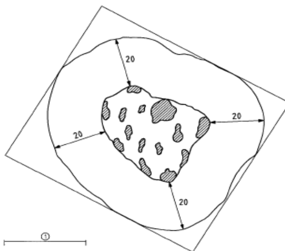
Figure 2 - Determination of the area influenced by clustered discontinuities (EN 10163-1:2004)
