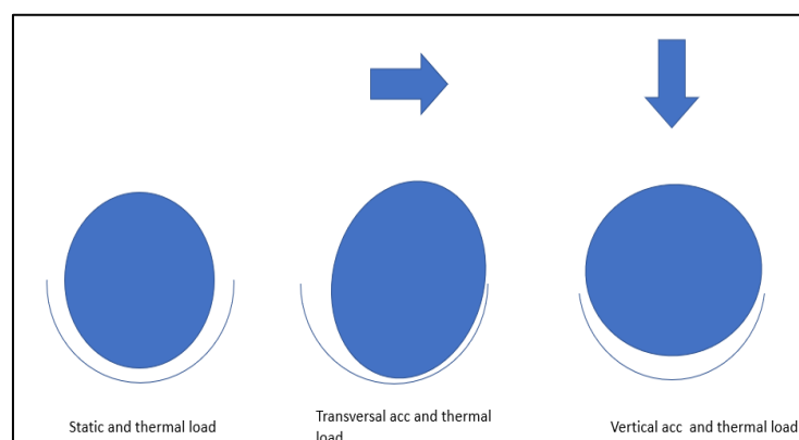
Figure 1 The figure illustrate the natural cylindrical tank deflections due to accelerations in transverse and vertical direction. The relative deflections between tank and supports may significantly affect the load distribution and the local stresses on the tank and the tank supports. A correct modelling of the contact between tank and support is therefore important to capture these effects.
