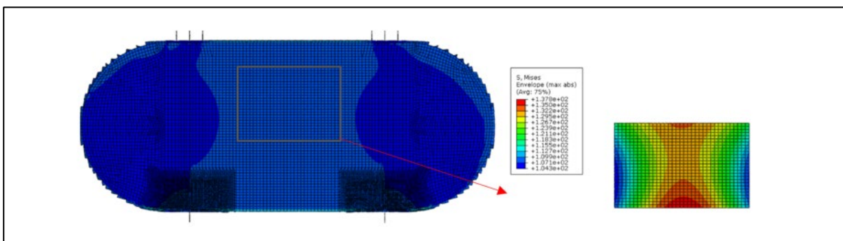
Figure 9 Stress contour for longitudinal bulkhe
