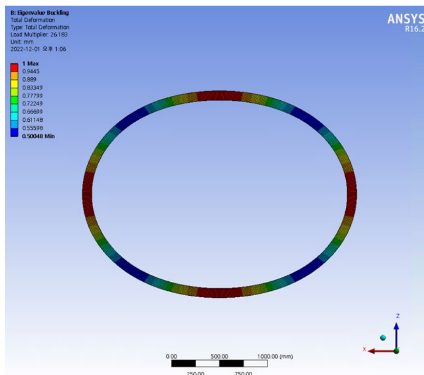
Figure 16 Buckling Mode of Stiffening Ring by Linear Buckling Analysis
