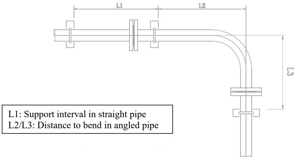
Figure 3 Pipe Support Interval
