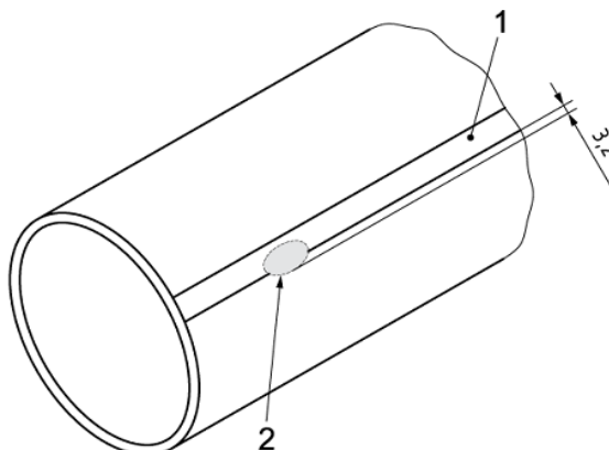
Figure 1 Resultant Cavity of Weld Repair (for class I and II)
