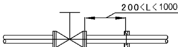
Figure 4 Distance between valve and pipe support
