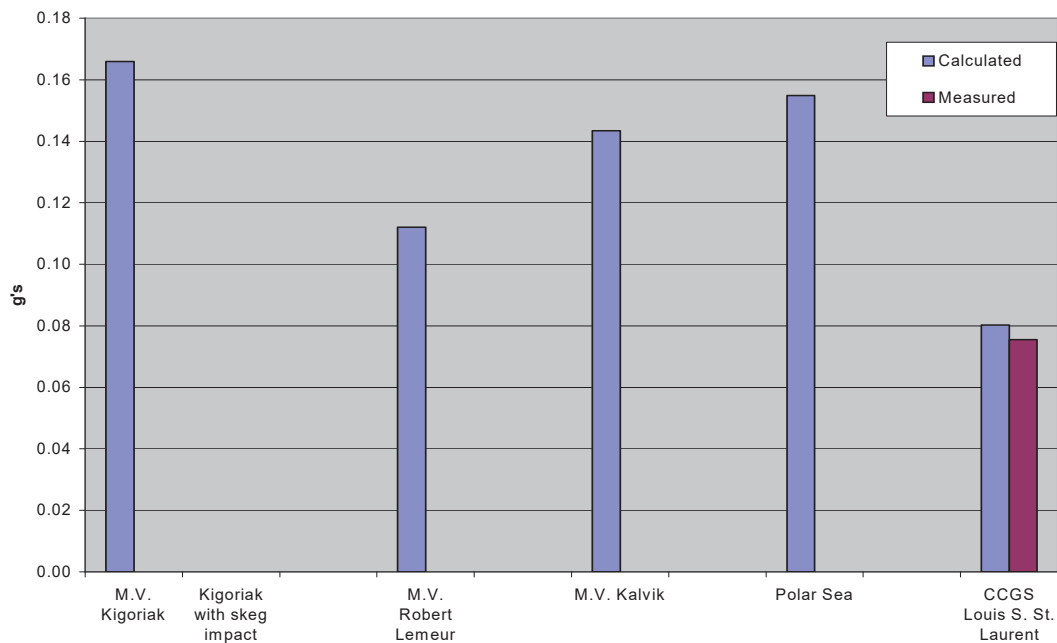
VERTICAL ACCELERATION AT MIDSHIPS IN ICE
