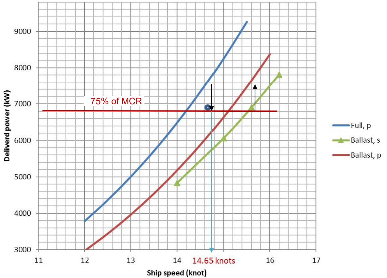
Figure 3.1: Power curves
